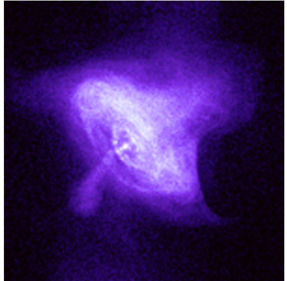
Crab Nebula, X-ray
