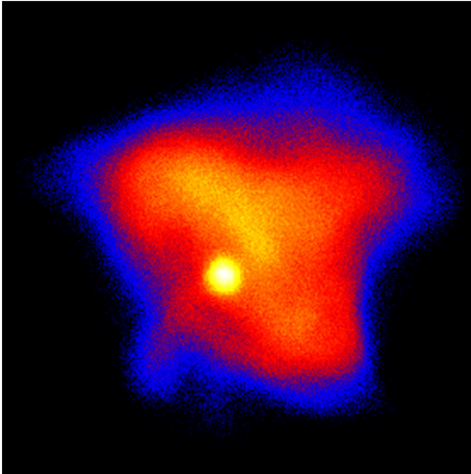
Crab Nebula, Rosat
