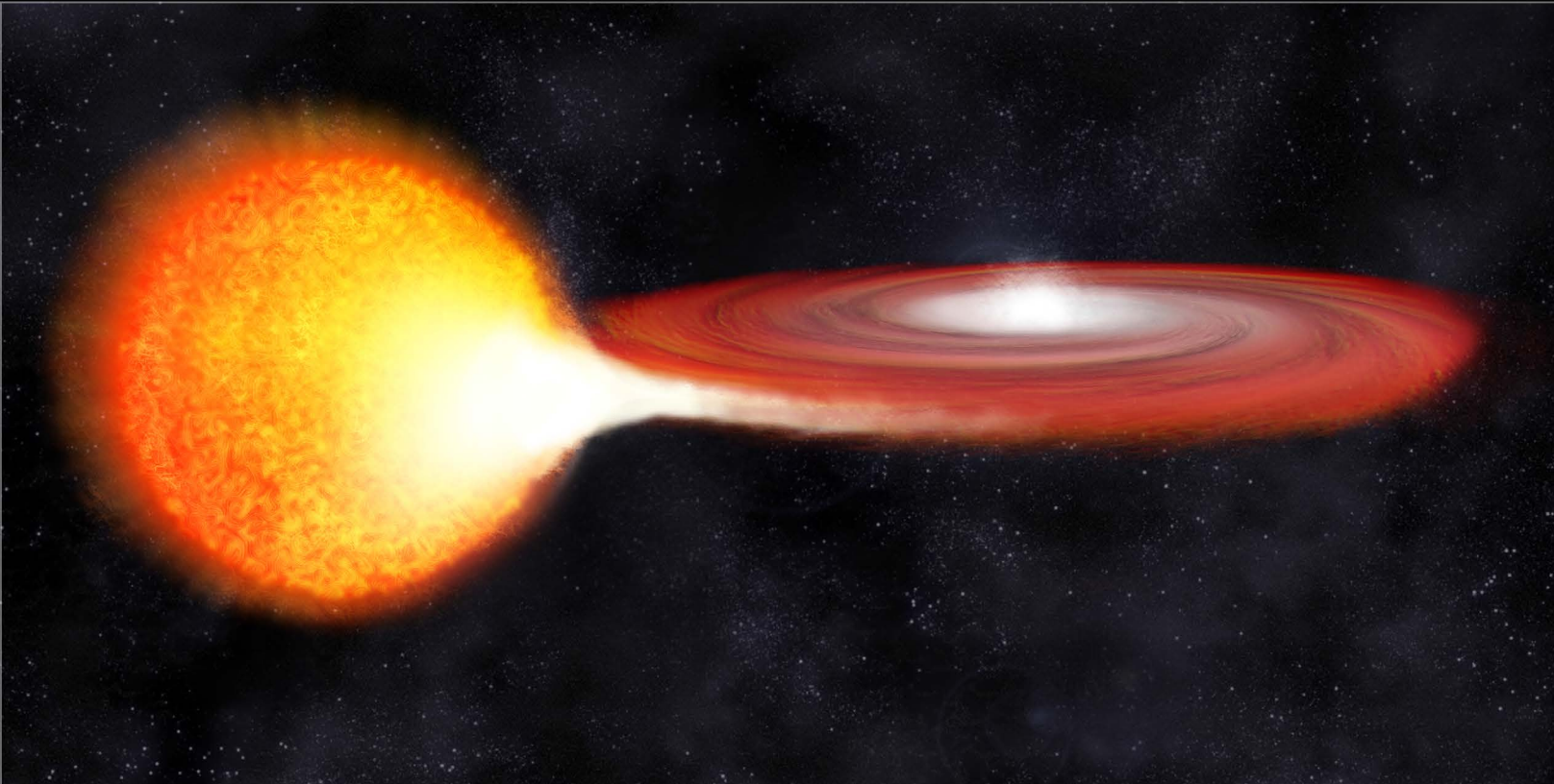
super-critical accretion onto a white dwarf star
