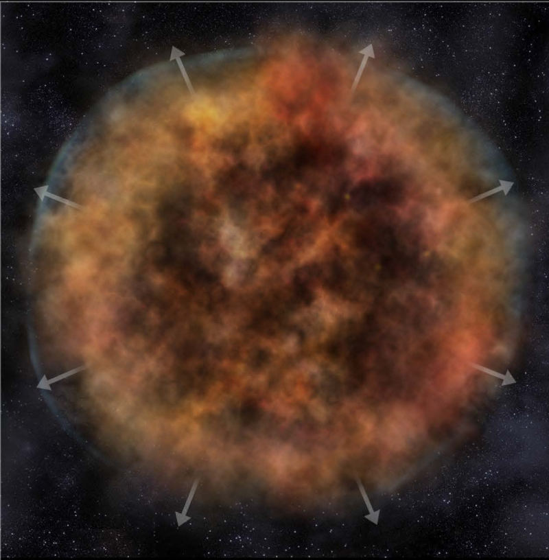
supernova remnant without a neutron star
