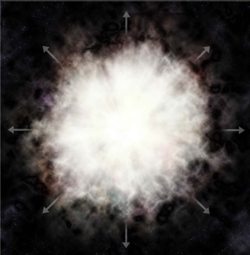
thermonuclear supernova explosion
