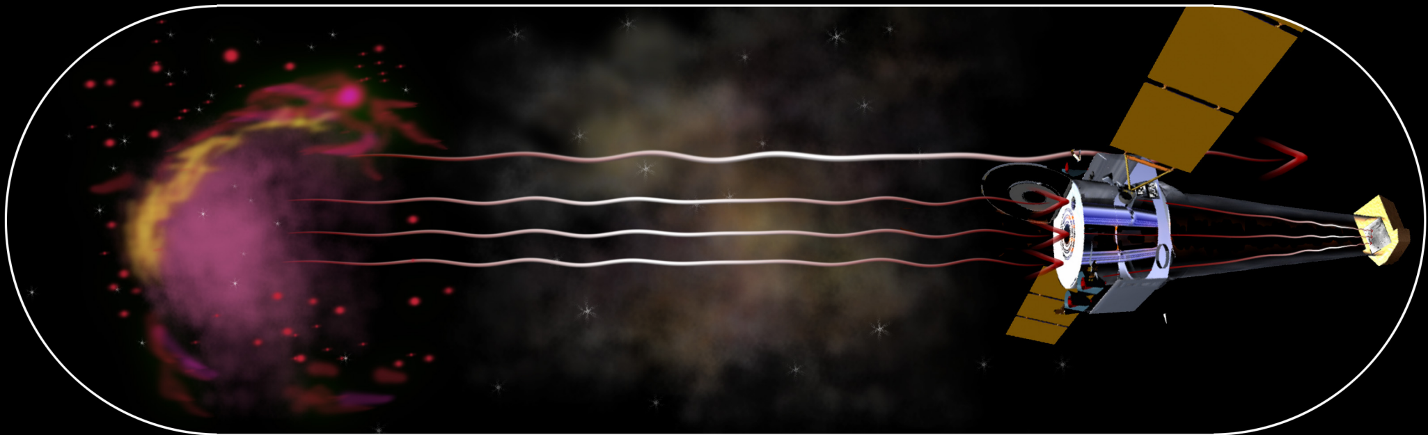
Galaxy
