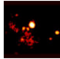
Chandra Image of M82 Black Hole
