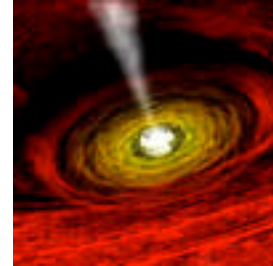
Schematic of a Black Hole
