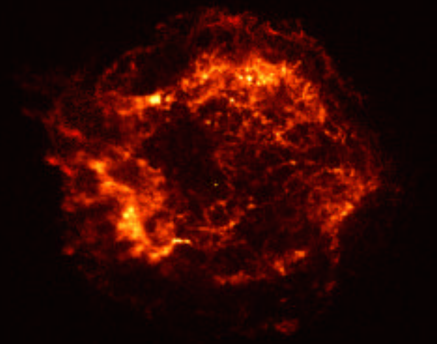
X-ray (NASA/CXC/SAO)
