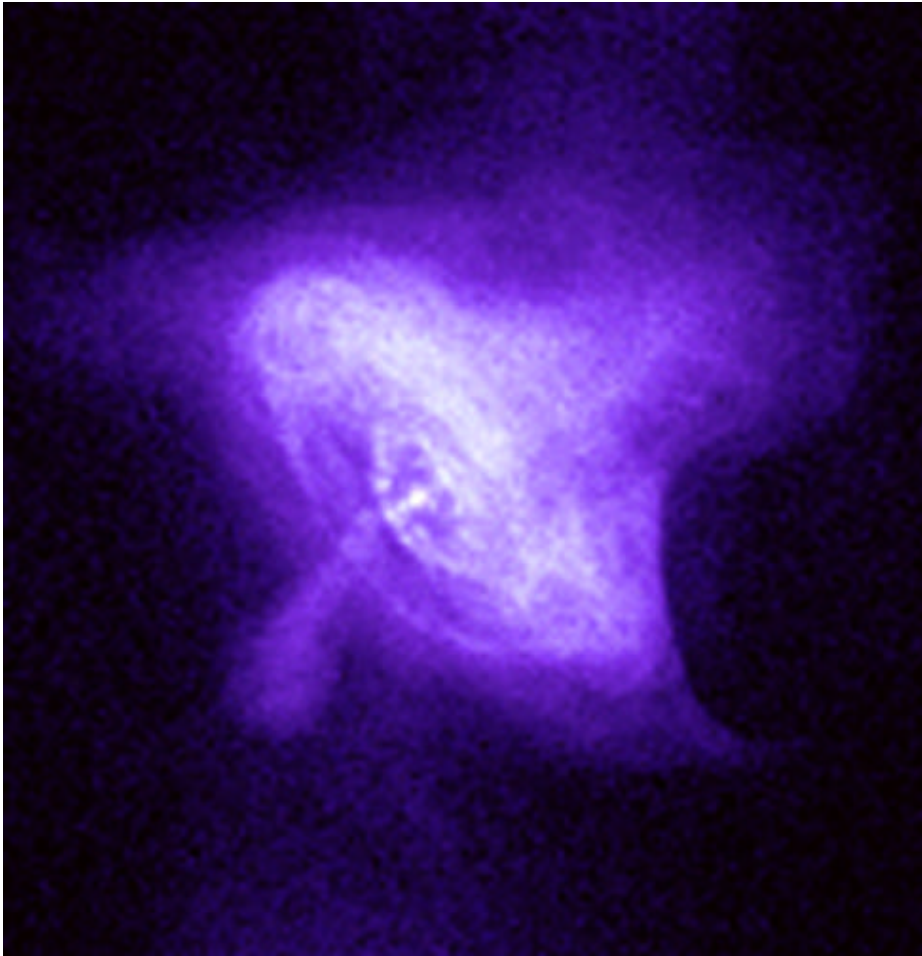
Crab Nebula
