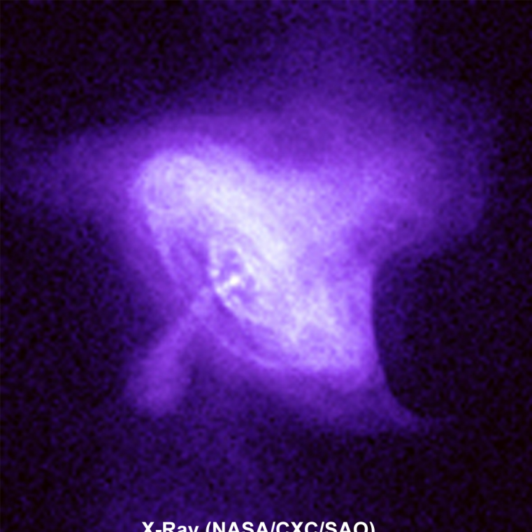
X-Ray (NASA/CXC/SAO)
