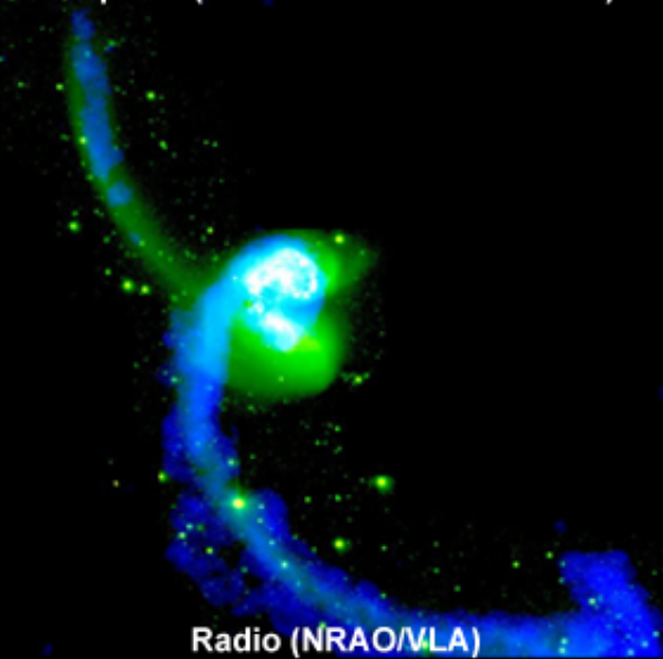
Optical (NASA/STScI/B.Whitemore)
